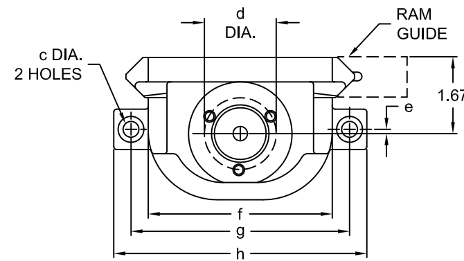
RAM DETAIL
